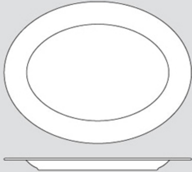
OVAL PLATTER U 2208 29.5 X 39.0 cm. (11 5/8" x 15 3/8") 907 g. U 2209 25.0 X 35.0 cm. (9 7/8" x 13 3/4") 706 g.
